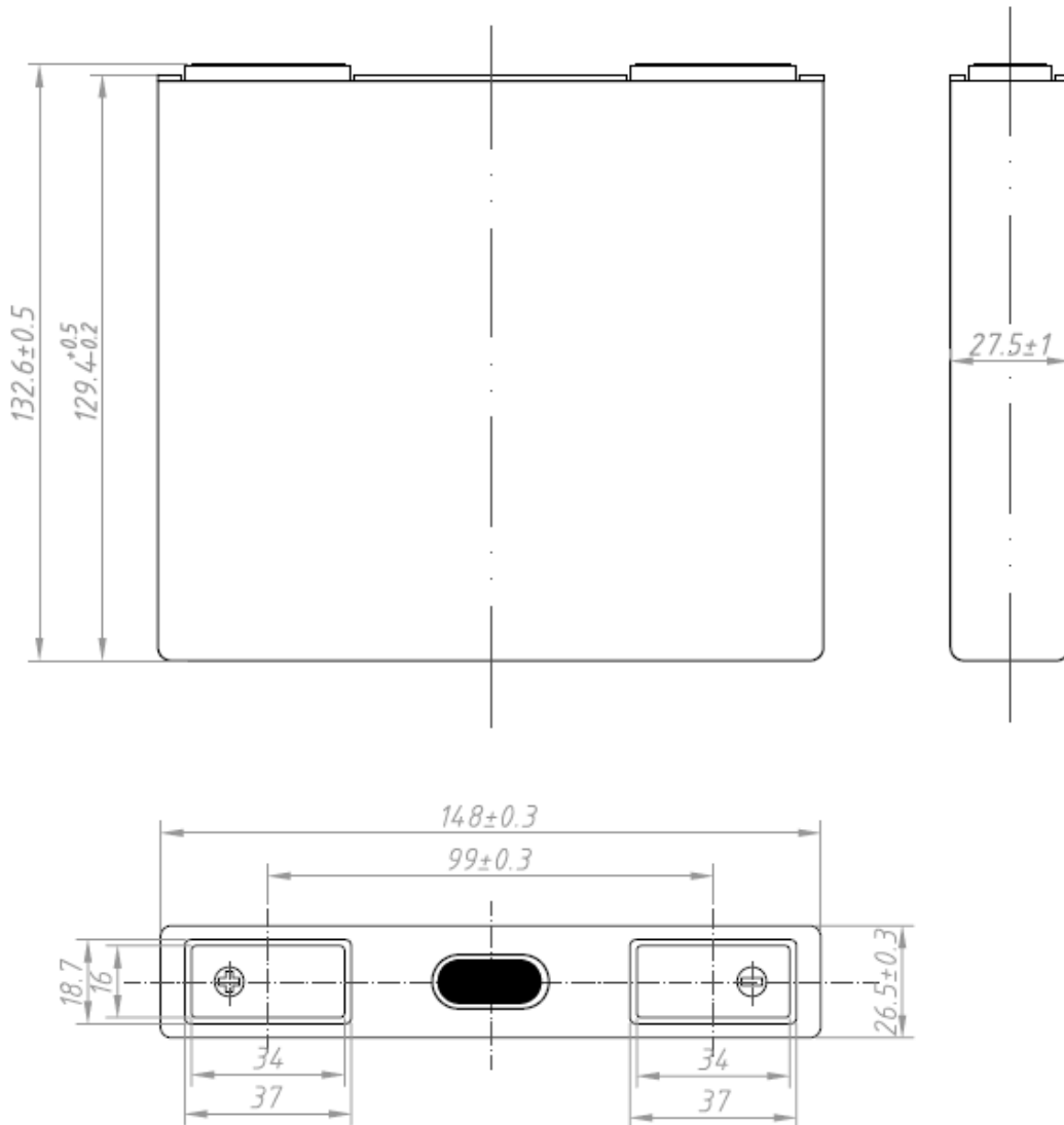
Drawing 1. Appearance and dimension of the battery
