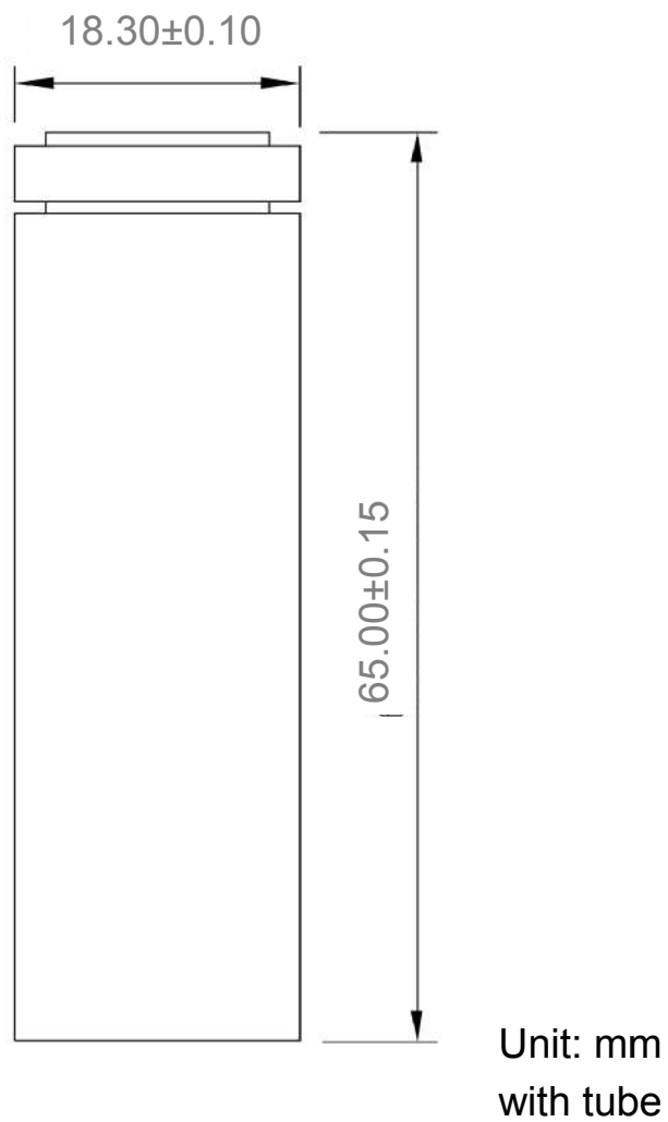
Fig. 1. Outline Dimensions of ICR18650/15P
